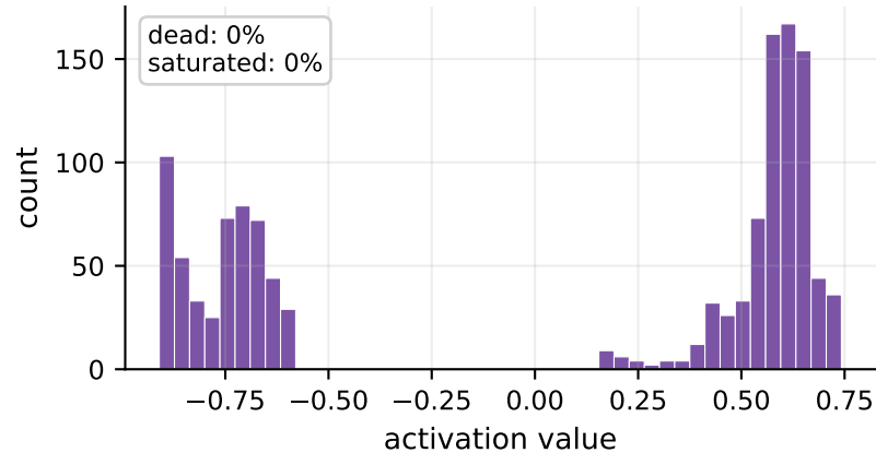
L1 (5 neurons)
