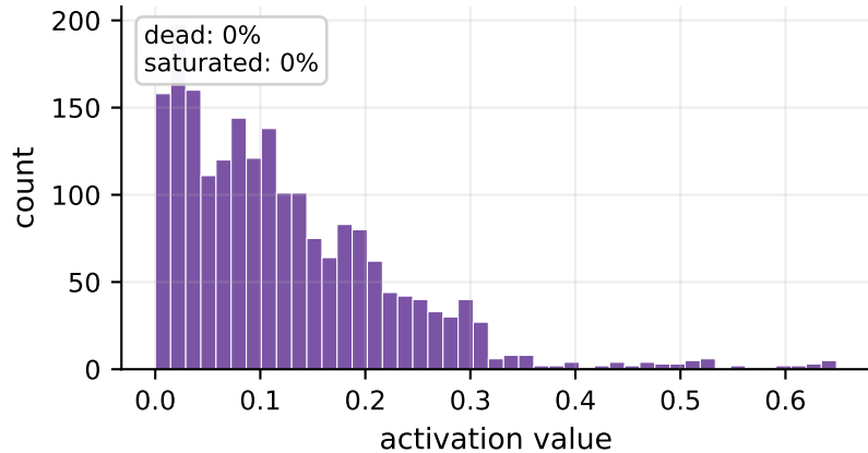
L0_quantum (8 neurons)
